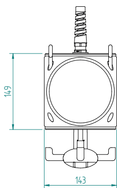
Suspended distributor, plastic
